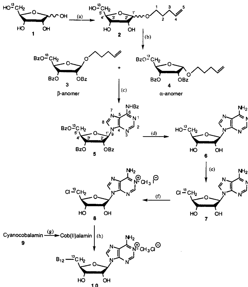
Scheme 1. Synthesis of {[A15- 13 C]5'-Deoxy-N1-methyladenosylcobalamin + }Cl - . (a) 4-pentenol, 10-camphorsulfonic acid, 48 h, RT; (b) benzoyl chloride, pyridine, RT, 24 h; (c) N 6 -benzoyl amino-purine, trifluoromethane sulfonic acid, CH 3 CN, RT, 2 h; (d) 0.1 N CH 3 ONa, reflux, 45 min; (e) thionyl chloride, hexamethylphosphoramide, RT, 15 h; (f) CH 3 I, dimethylacetamide, RT, 20 h; (g) Zn, 10% NH 4 Cl, Ar, RT; (h) cob(II)alamin, RT.
