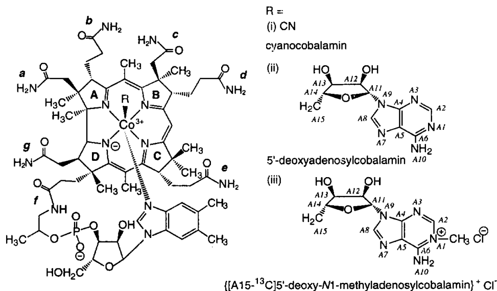
Figure 1. Structures of (i) Cyanocobalamin, (ii) Coenzyme \text{B}_{12} (5'-deoxyadenosylcobalamin), and (iii) \{[A15-^{13}\text{C}]5'-\text{deoxy-}N1\text{-methyladenosylcobalamin}^+\}\text{Cl}^- .
